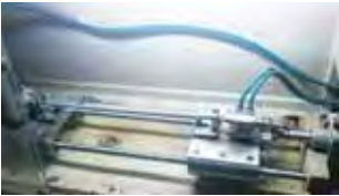
Spiral Su, Sıcaklık ve Burkulma Testi / Shower Hose Tension and Flowrate Testing
